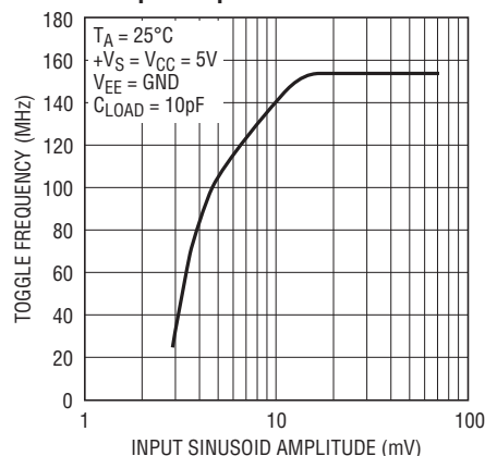
Maximum Toggle Rate vs Input Amplitude
