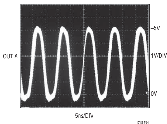
Figure 4. 100MHz Jitter with Both Channels Driven
