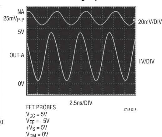
Response to 150MHz 25mVp-p Sine Wave Driving 10pF
